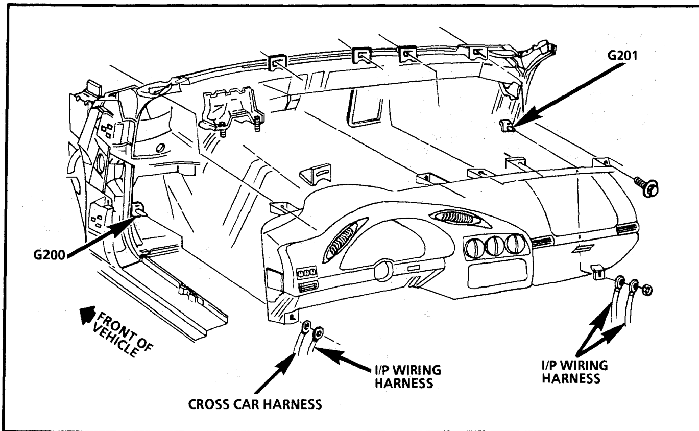
Figure 16 - I/P Grounds (Chevy shown Pontiac similar)
