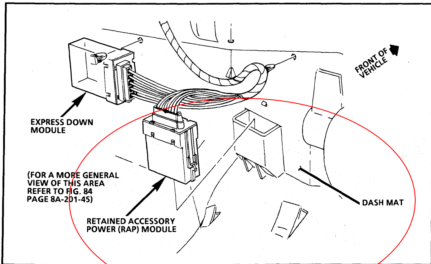
Figure 17 - Center of Dash Mat Above Floor Tunnel
