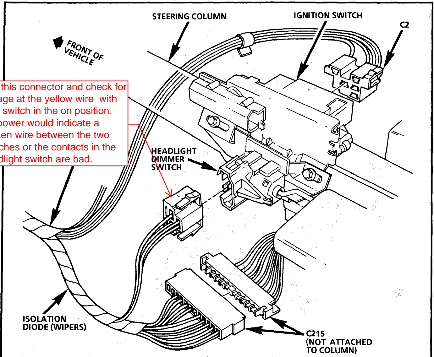
Figure 64 - Bottom of Steering Column
