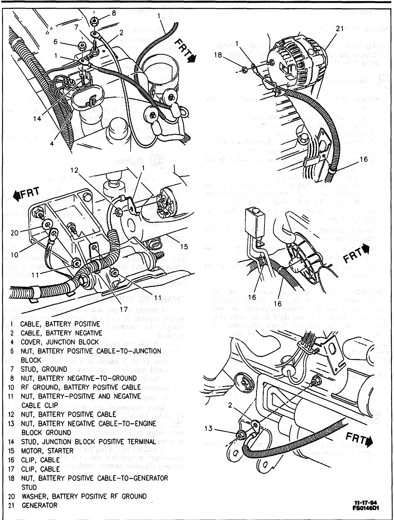
Figure 10 - Battery Cable Routing (3800 VIN K)
