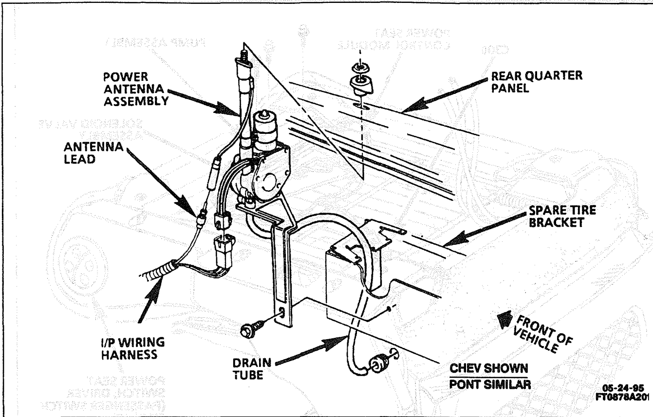
Figure 87-Behind Right Rear Interior Quarter Trim Panel
