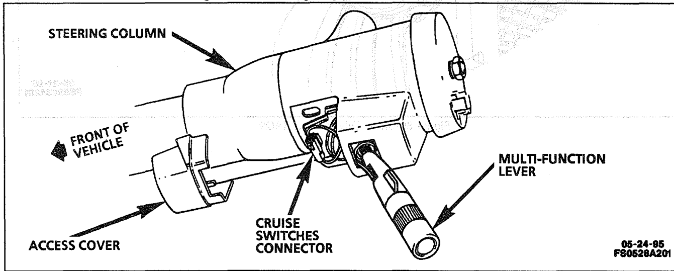
Figure 88-Steering Column
